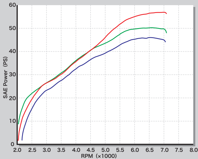
W800 ■ 814cc Piston Kit+Stock camshaft+Original Exhaust system ■ 814cc Piston Kit+Stock camshaft+Stock Exhaust system ■ Stock Engine+Stock Exhaust system ※ To prevent the engine from getting damaged, keep specified rpm range. ※ Tested at the condition of our test facility, actual power may vary.
