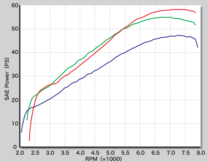
W650 ■ 814cc Piston Kit+Stock camshaft+Original Exhaust system ■ 814cc Piston Kit+Stock camshaft+Stock Exhaust system ■ Stock Engine+Stock Exhaust system ※ To prevent the engine from getting damaged, keep specified rpm range. ※ Tested at the condition of our test facility, actual power may vary.
