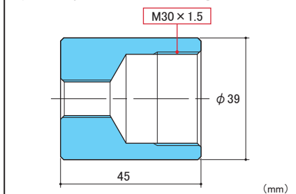
Flywheel puller detail drawing
