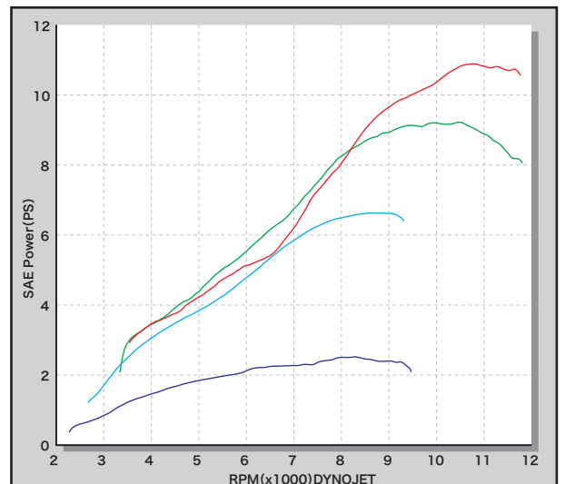
Big throttle body kit
