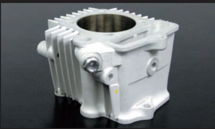
Ceramic plated cylinder (for 138cc)
