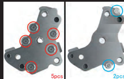
Comparison of the number of bolts Left: Super oil pump Right: Stock pump
