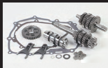
TAF 5 speed close ratio transmission kit (Exclusive use for Special / Dry clutch TYPE-R)
