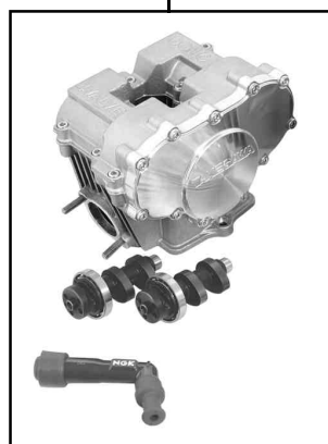
01-03-6008 DOHC Kit
