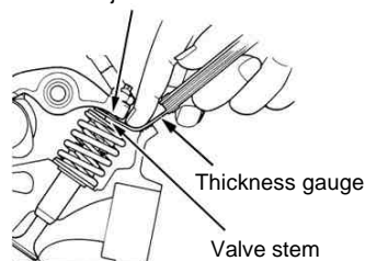
Adjust screw
