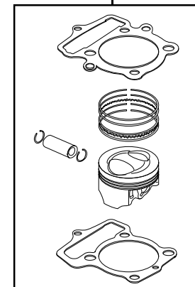
01-02-0129 53 Piston kit
