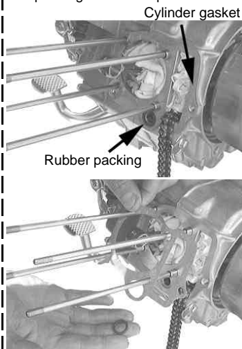
Cylinder gasket
