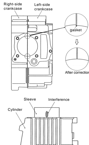
Cylinder gasket
