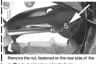
Remove the hex nut securing the muffler by turning it counterclockwise. Tool to use Socket, 12 mm Extension (medium)
