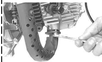
Remove two nuts on the exhaust pipe by turning them counterclockwise. Tool to use Open-end wrench, 10 mm
