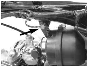
Unfasten a bolt on the air-cleaner stay. Tool to use Socket, 10 mm Extension (short)
