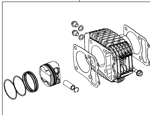
01-04-0130 Cylinder Kit (181cc)
