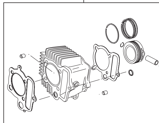
01-04-7004 Cylinder kit 106cc(SCUT Clinder)
