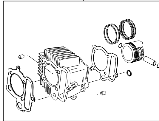
01-04-7088H Cylinder kit 88cc (H Cylinder)
