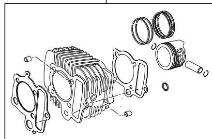
01-04-8088V 88cc V Cylinder kit
