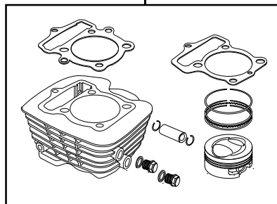
01-04-1017 62 SCUT Plated Cylinder kit
