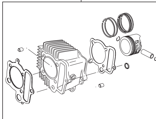
01-04-7106H Cylinder kit 106cc (H Cylinder)
