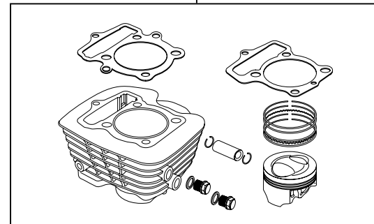
01-04-1012 Big Fin Cylinder Kit 120/130cc
