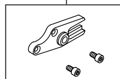
06-08-0026 Rear caliper bracket kit (Rigid type)
